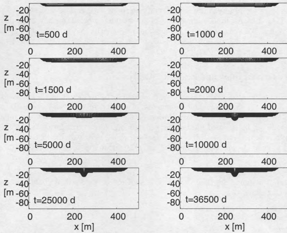
Figure 2: Concentration isolines modelled without density coupling
