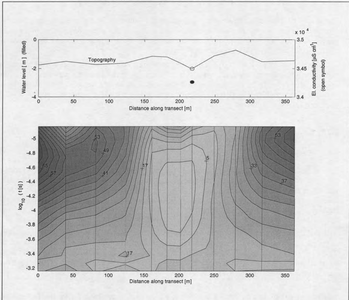
Figure 5: Thata Island Transect 1 with topography, water level and electrical conductivity (top), late apparent resistivity [ \Omega \text{ m} ] (bottom)
