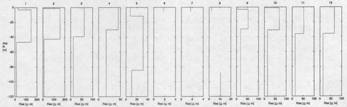
Figure 7: Modelling results for Thata Island Transect 1
