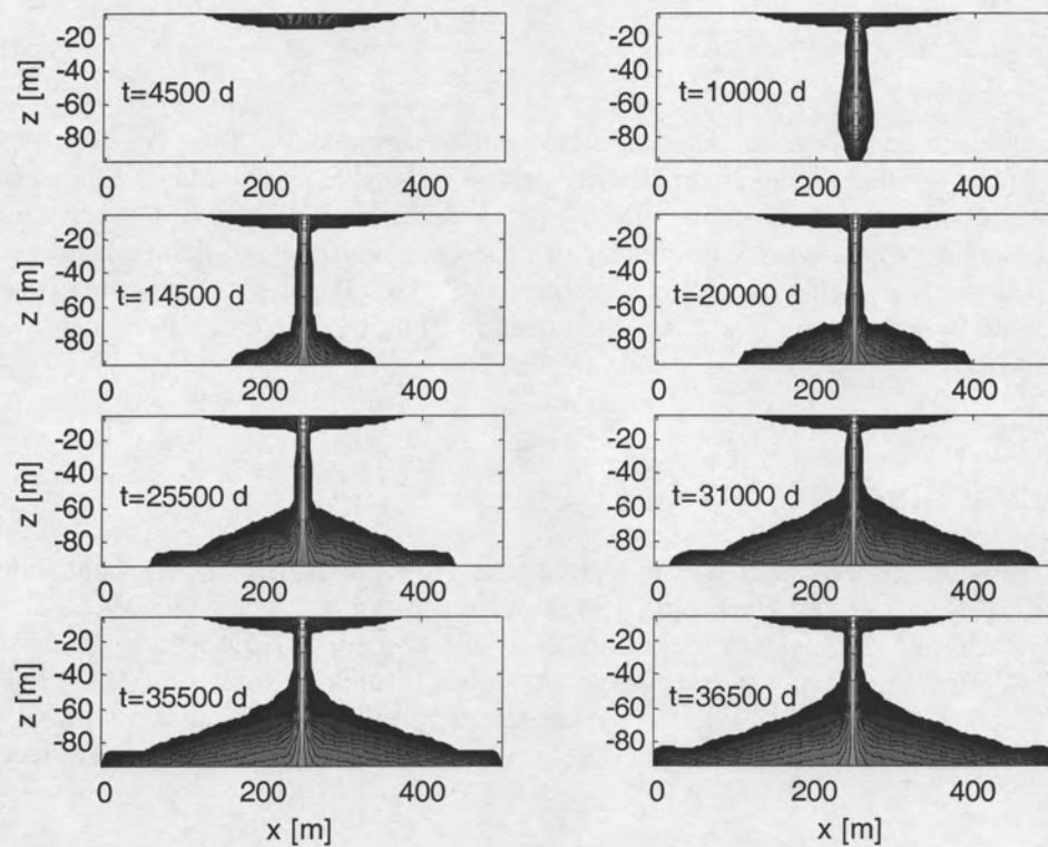
Figure 3: Concentration isolines modelled with density coupling
