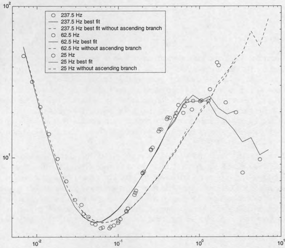
Figure 6: Measured data and modelling responses for Thata Transect 1 Sounding 7 (see text for explanation)
